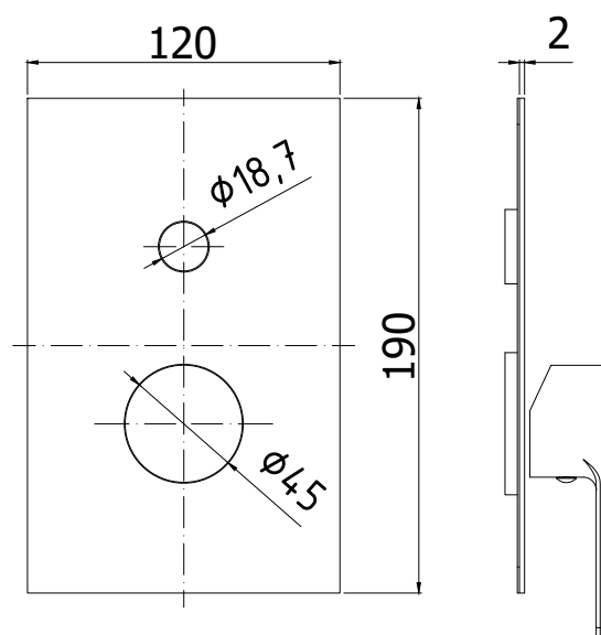
TECHNICAL DRAWING
