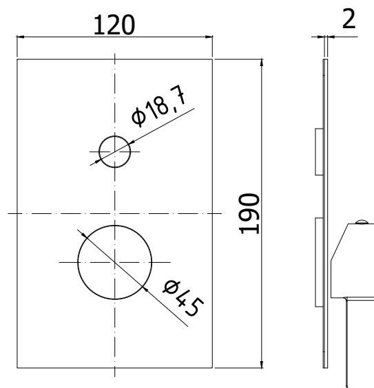
TECHNICAL DRAWING
